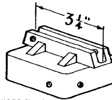
#850 Short Available for both Flat & Extruded Blades Cap for 2" Square Tube 5/16" Set Screw - 6 Places
