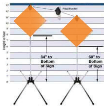
4860RBK 11'2" and 13'2" deployed height 5' and 7' ground to sign
