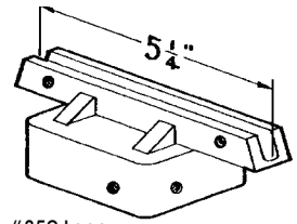
#850 Long Available for both Flat & Extruded Blades Cap for 2" Square Tube 90 Crosspiece Slot 5 1/4" Long 5/16" Set Screw - 6 places
