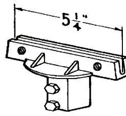
#808EX - Available for both Flat & Extruded Blades U-Channel Cap **Extruded Opposite Cap also available 5/16" Set Screw
