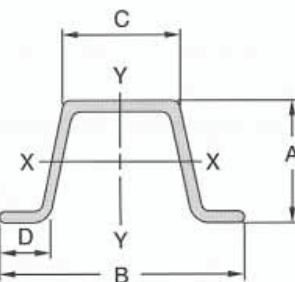
Sign Post and Base Post Weight - 3.00 lbs/ft
