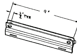
#850 Long Available for both Flat & Extruded Blades Cap for 2" Square Tube 90 Crosspiece Slot 5 1/4" Long 5/16" Set Screw - 6 places
