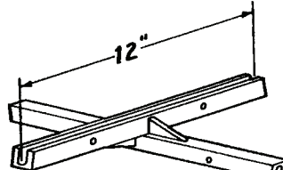
5/16" Set Screw - 4 Places
